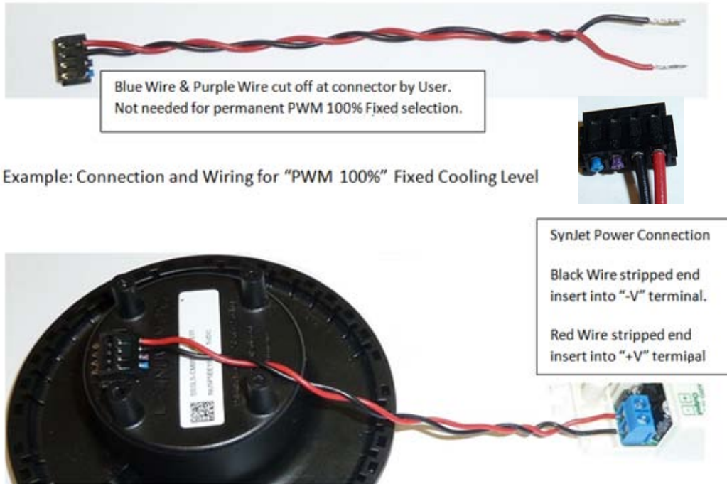
Figure 3. Permanent PWM 100% or CVC Maximum Cooling Level Selection
