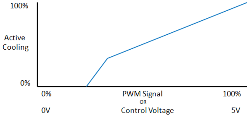
Figure 1. SynJet Active Cooling versus User Input Signal
