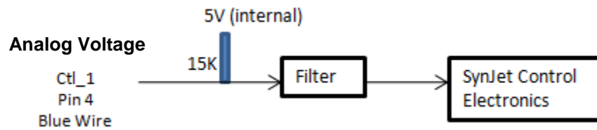
Figure 4. SynJet “Analog Voltage” Control Input Circuit
