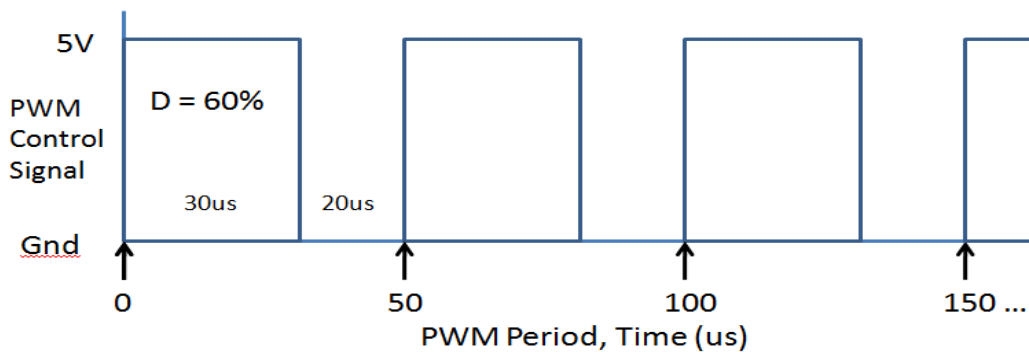
Figure 2. PWM Control Signal - User System to SynJet Pin 4 (Blue Wire)
