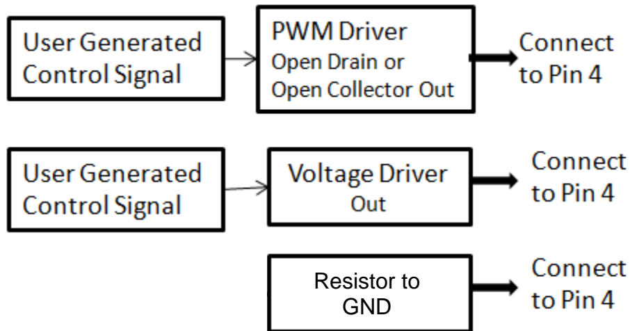
Figure 5. User Control Signal Output – Typical User Circuits
