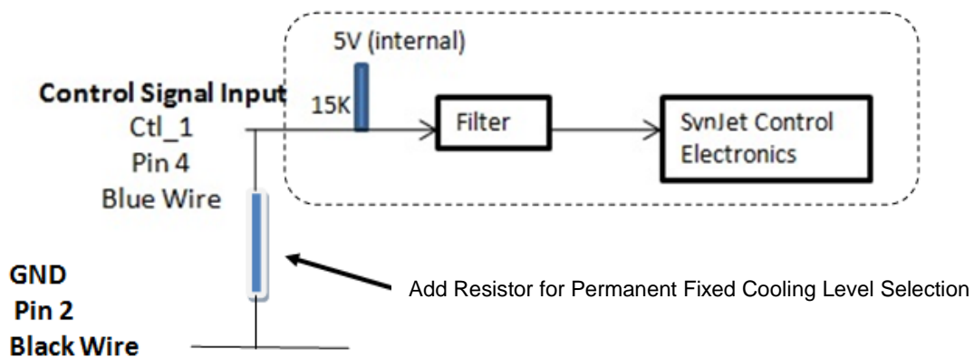
Figure 6. Block Diagram – Fixed Resistor and Pin 4 Connection
