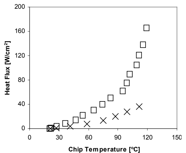
Figure 8. The heat flux from the thermal test die with the jet on ( \square ) and with the jet off ( x ).
