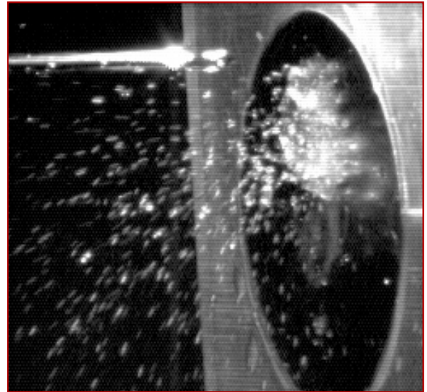
Figure 10a. Ejected secondary droplets with the atomizer in a vertical orientation. The supply tube is normal to the atomizer.
